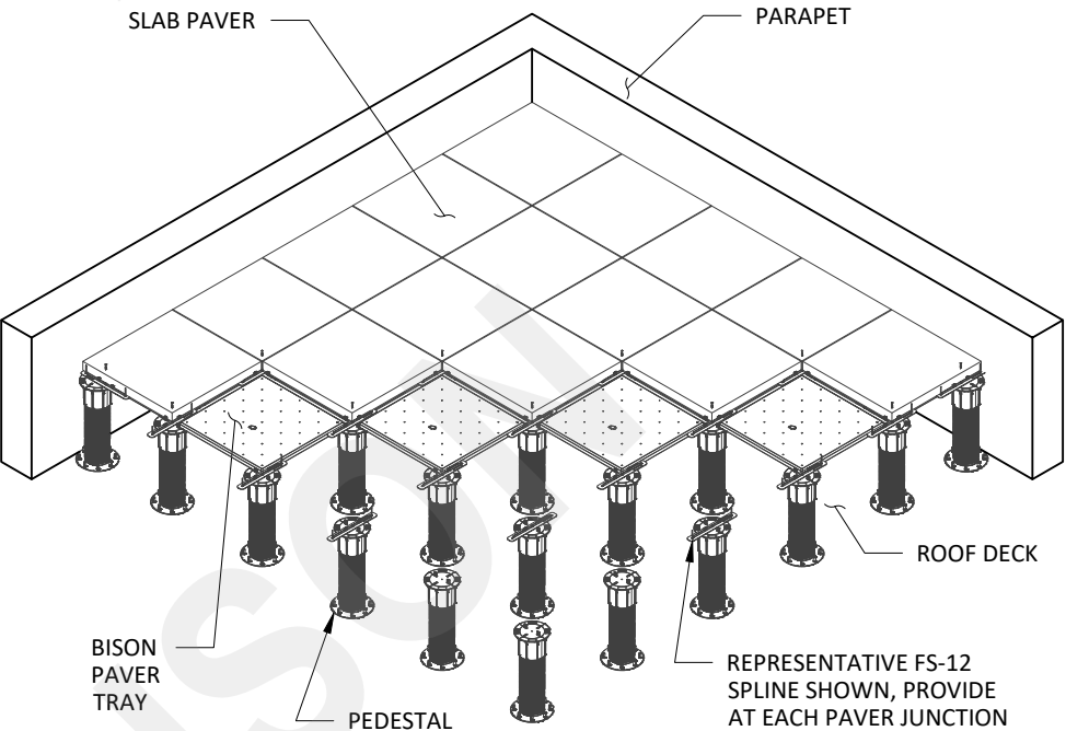
F1 BISON PAVER TRAY/SLAB PAVER SYSTEM ISOMETRIC NTS
