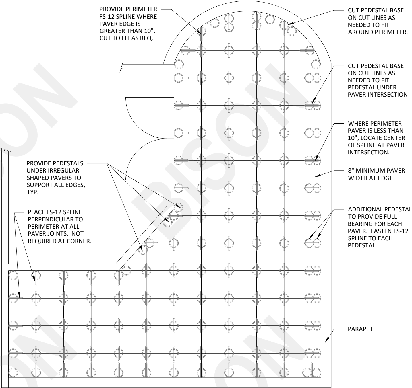
D8 BISON PAVER TRAY/SLAB PAVER SYSTEM LAYOUT DIAGRAM SCALE: 1/4" = 1'-0"
