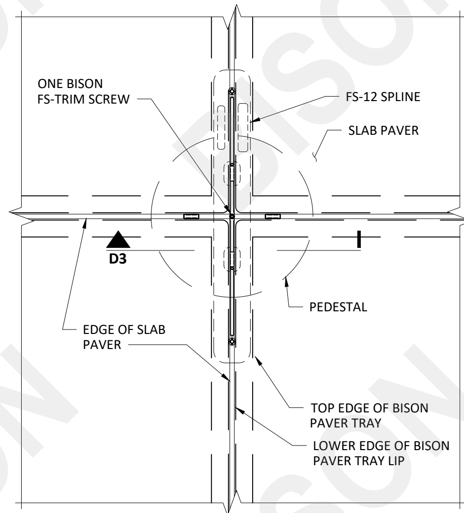
D2 FS-12 SPLINE CONNECTION - PLAN VIEW SCALE: 3" = 1'-0"
